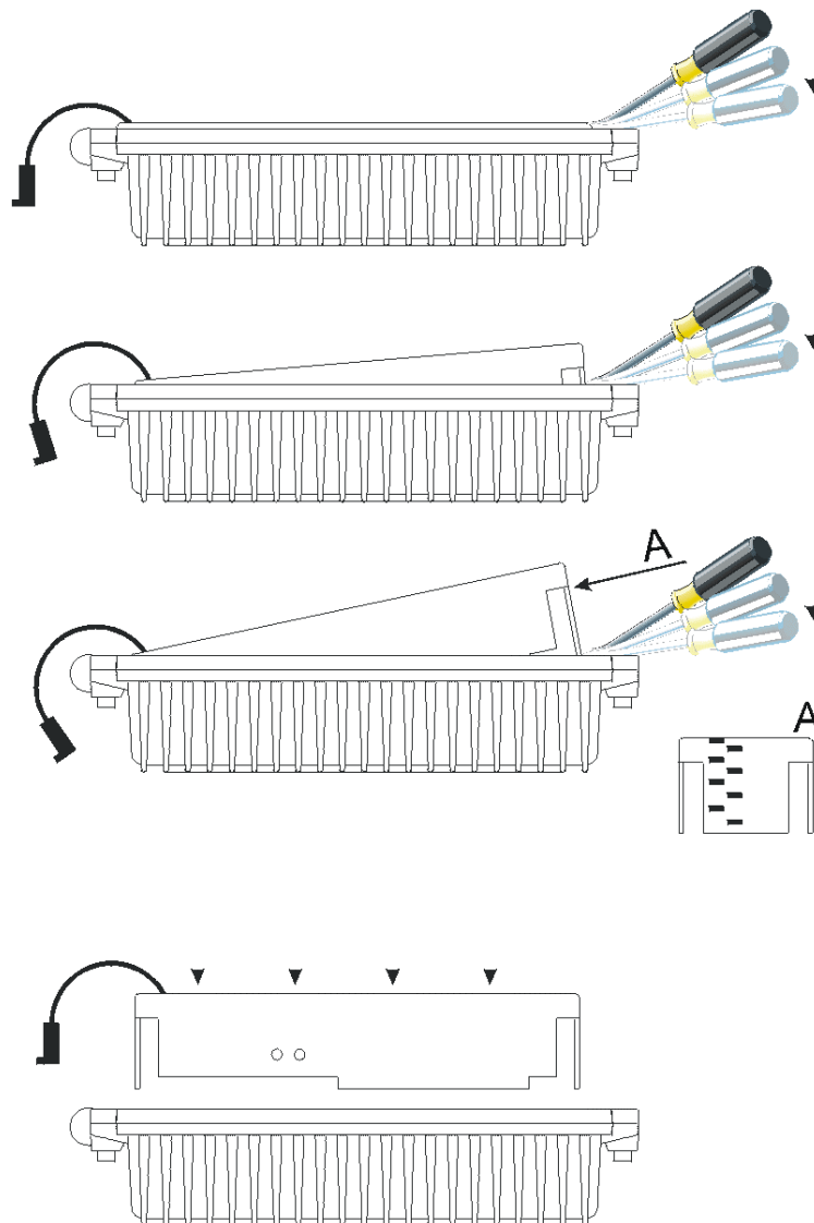
Fig. 9. SMPS module dismounting.
