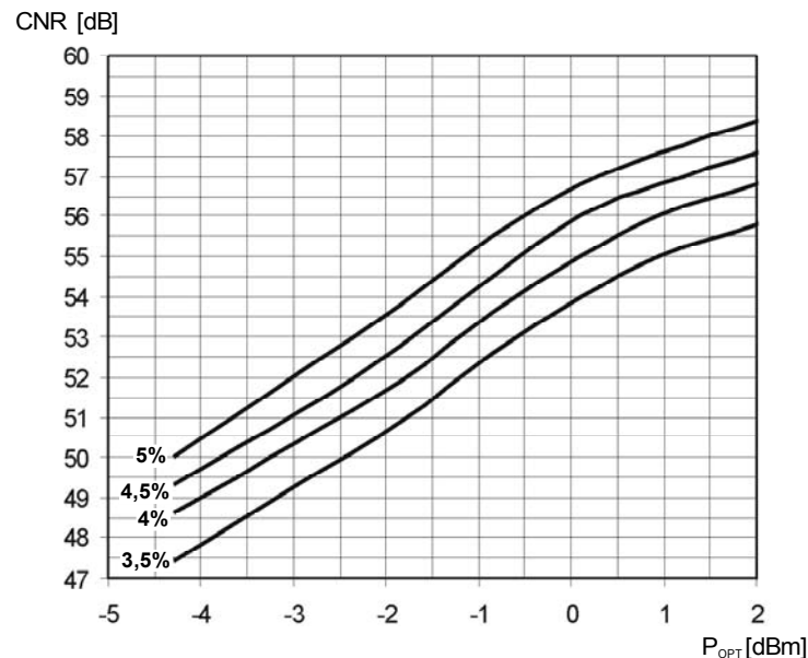
Fig. 20. CNR vs. optical input power and OMI/channel.
