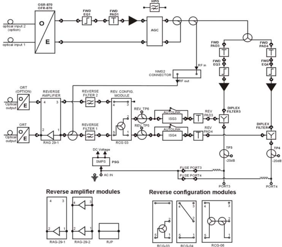
Fig. 2. GAMMA O8X-22A-AE8 optical node functional block diagram.
