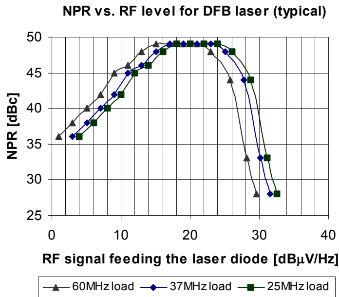
Fig. 25. NPR vs. RF level drive for optical reverse transmitter ORT D1310-xxx (typical).
