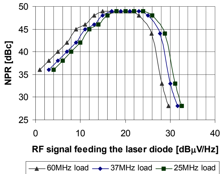
Fig. 24. NPR vs. RF level drive for optical reverse transmitter ORT D1310-xxx (typical).
