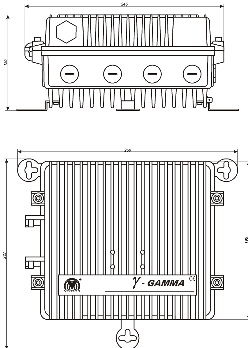
Fig. 7. An overview of GAMMA optical node's housing.
