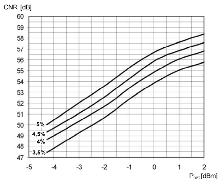
Fig. 19. CNR vs. optical input power and OMI/channel.
