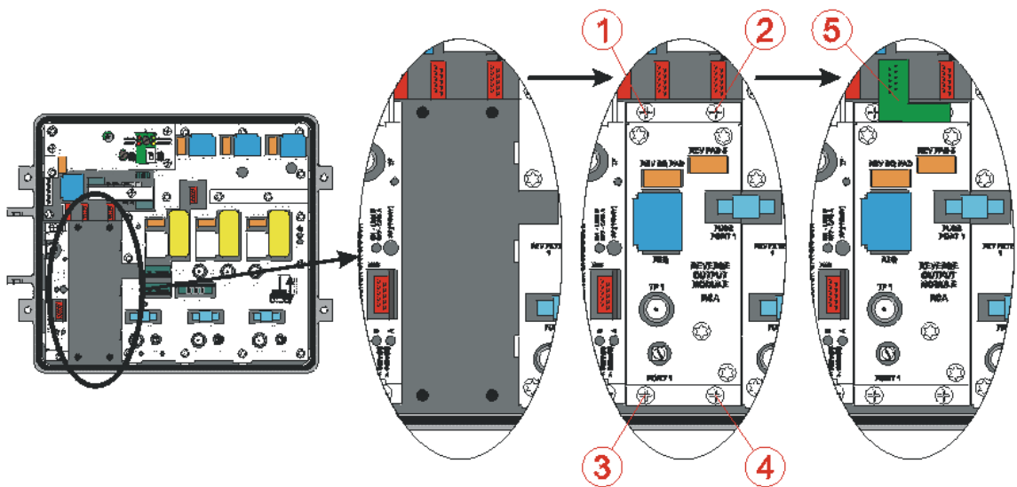
Fig. 11. RCA module installation.
