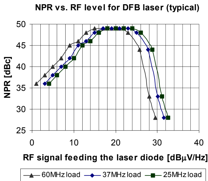
Fig. 22. NPR vs. RF level drive for optical reverse transmitter ORT D1310-xxx (typical).
