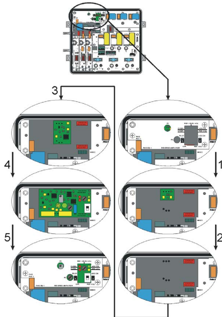
Fig. 10. AGC module mounting.
