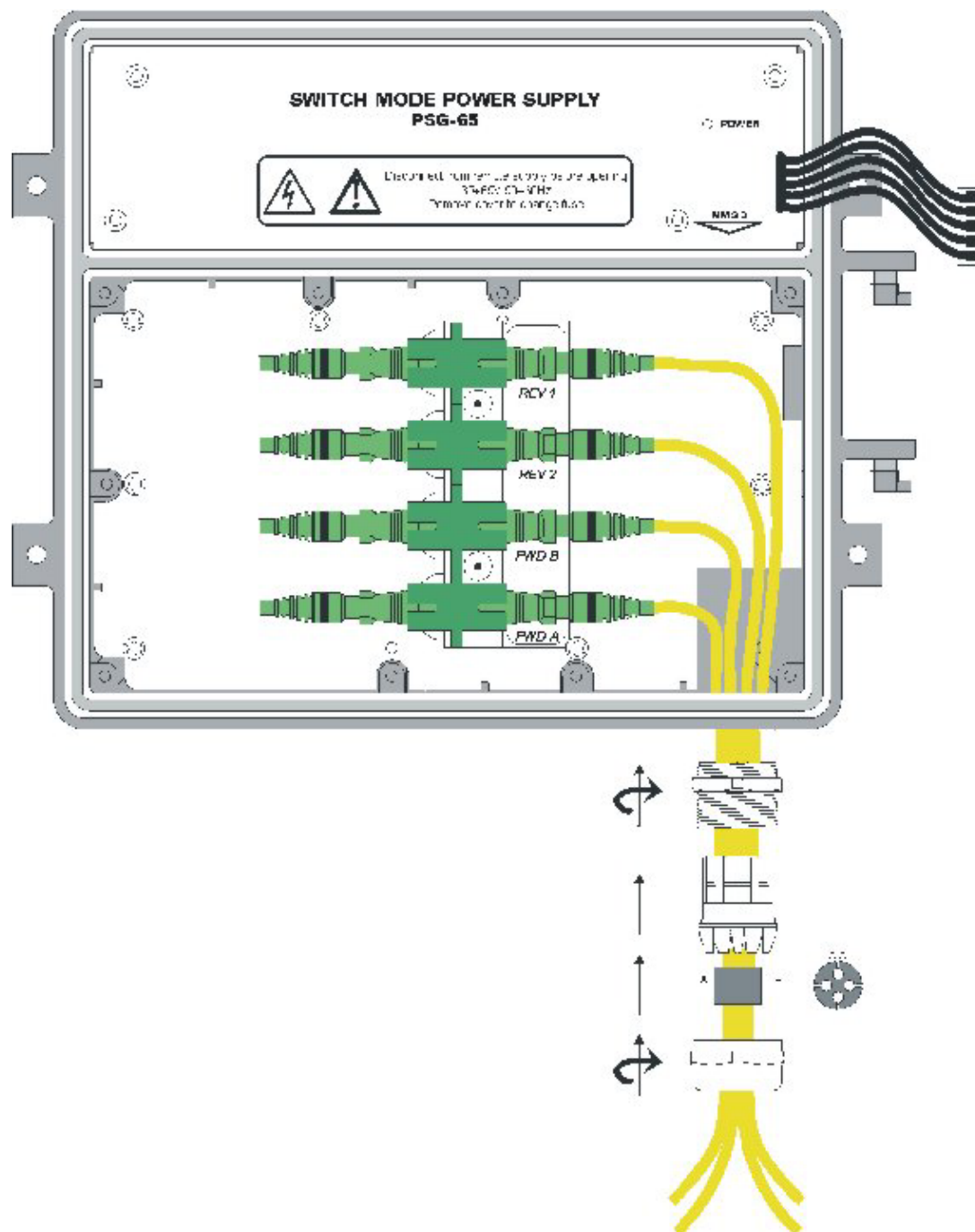
Fig. 8. Fiber connectors installation.
