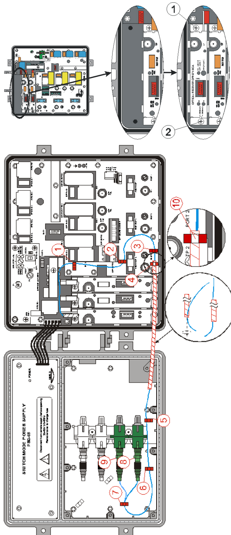
Fig. 15. Optical receiver with redundancy module OSR installation.
