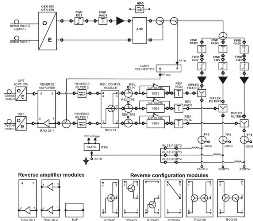
Fig. 3. GAMMA O8X-33A-AF8 optical node functional block diagram.
