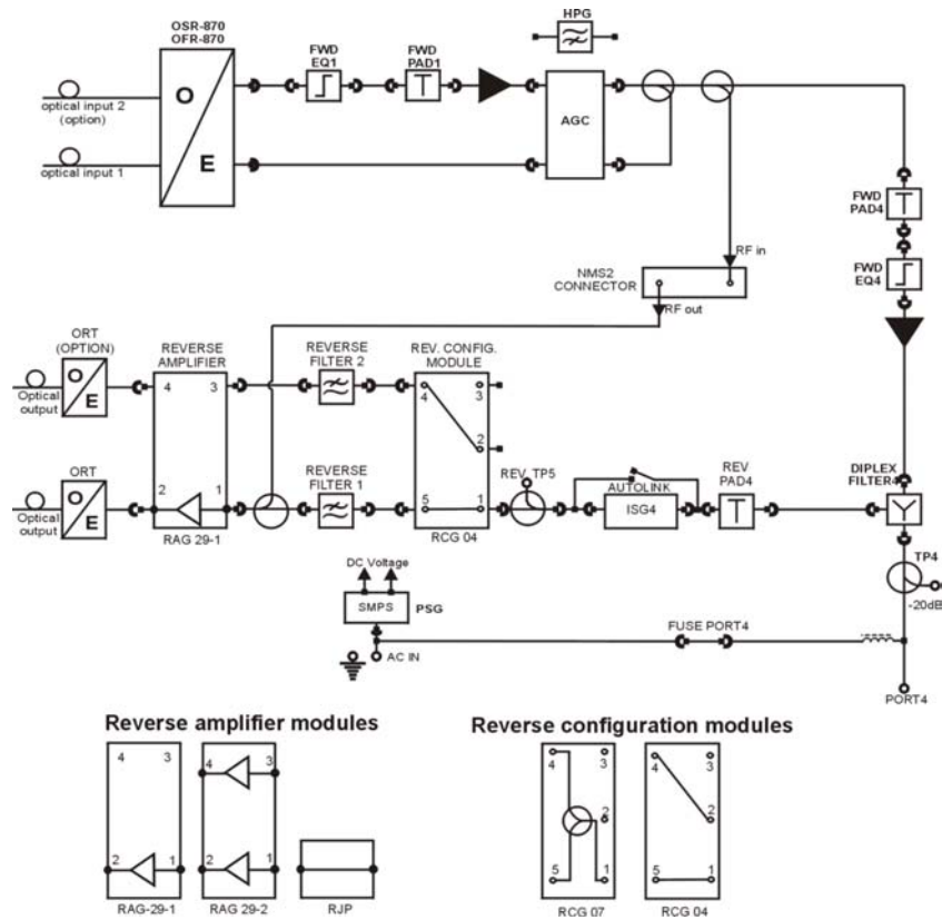
Fig. 1. GAMMA O8X-11A-AE8 optical node functional block diagram.
