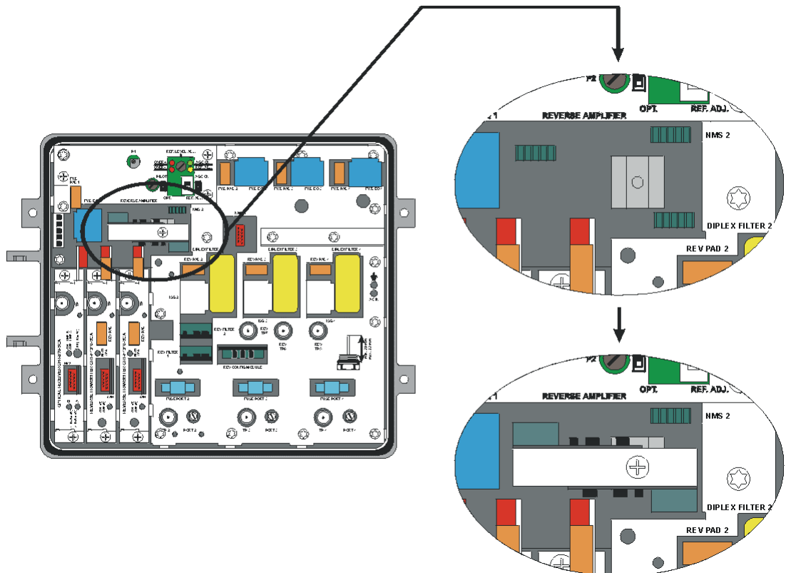
Fig. 13. RAG 29-x module mounting.
