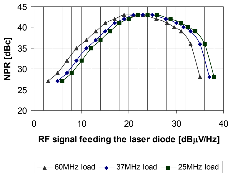
Fig. 21. NPR vs. RF level drive for optical reverse transmitter ORT F1310-xxx (typical).
