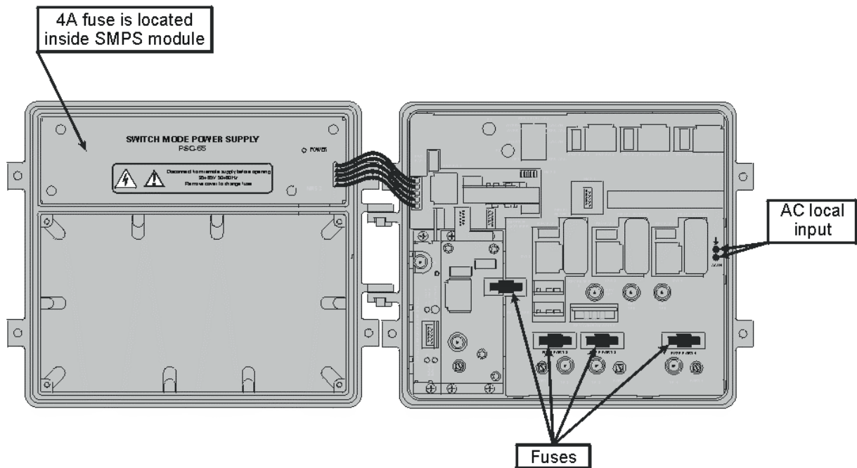
Fig. 4. Fuses location.
