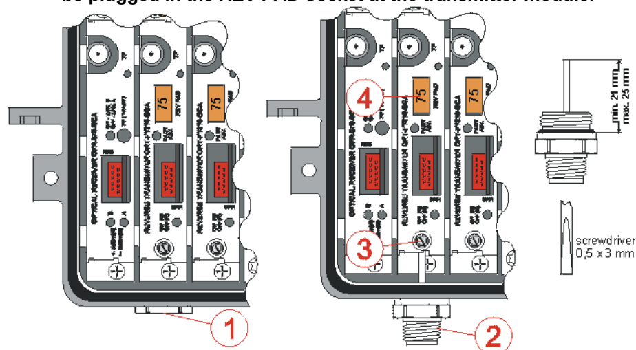
Fig. 18. External reverse RF 5 ÷ 210MHz input activation
