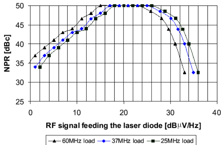
Fig. 23. NPR vs. RF level drive for optical reverse transmitter ORT 3D1310-xxx (typical).
